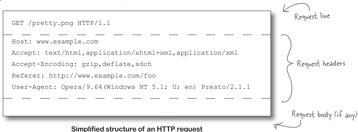
Simplified structure of an HTTP request
