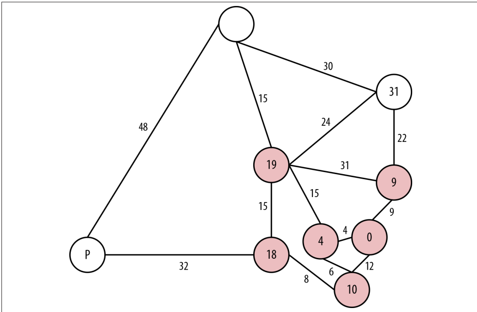
Figure 7-8. Taking a “detour” through Alice Springs
