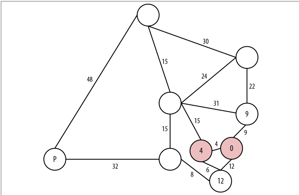
Figure 7-4. Canberra is the closest city to Sydney
