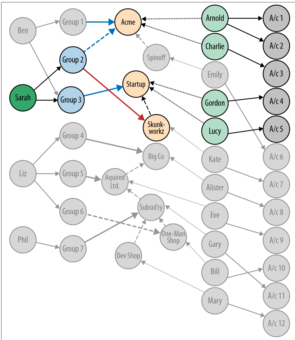
Figure 5-9. Finding all accessible resources for a user
